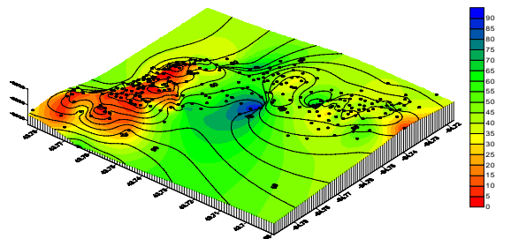
Top of Porosity Overlaid by Limestone Cap
