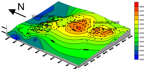
Top of Dundee
