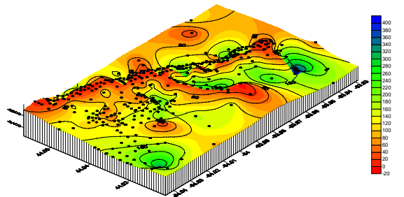
Top of Porosity Overlaid by Limestone Cap
