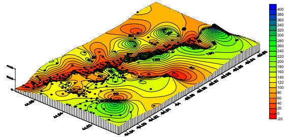
Thickness of Limestone Cap
