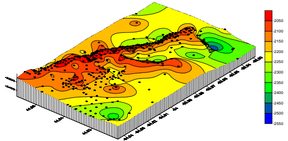
Top of Dundee Porosity
