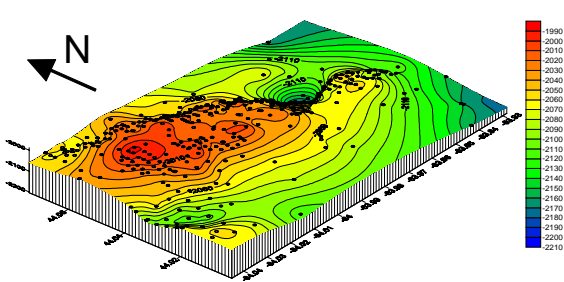
Top of Dundee
