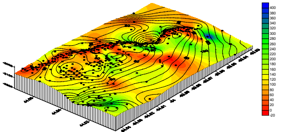
Top of Dundee Overlaid by Limestone Cap
