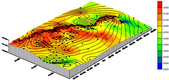
Top of Dundee Overlaid by Top of Porosity
