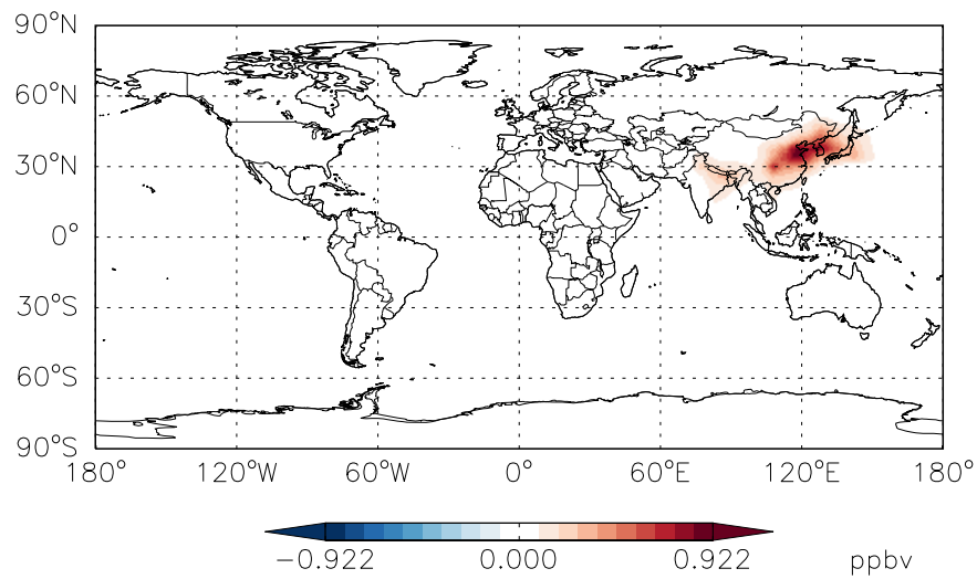
DIFF BCPO at Level 1
