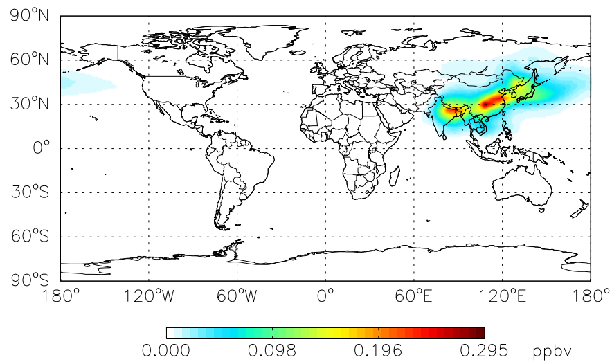
BCOC3 BCPO at Level 23
