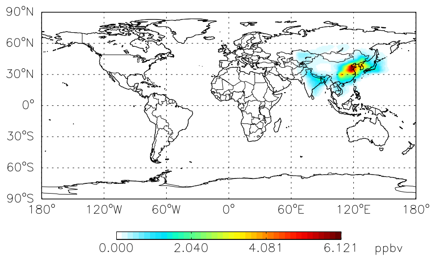
BCOC3 BCPI + BCPO at Level 1
