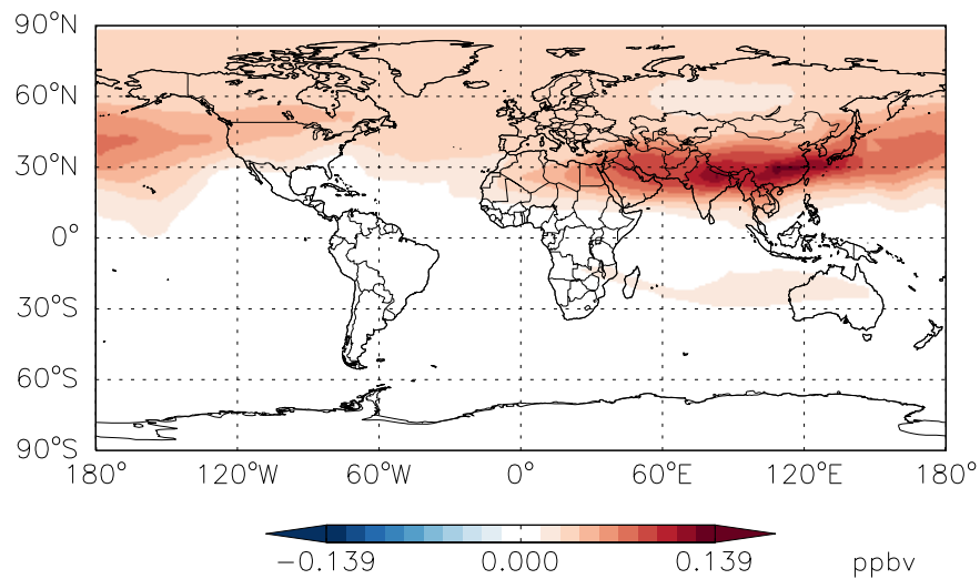
DIFF BCPI + BCPO at Level 30
