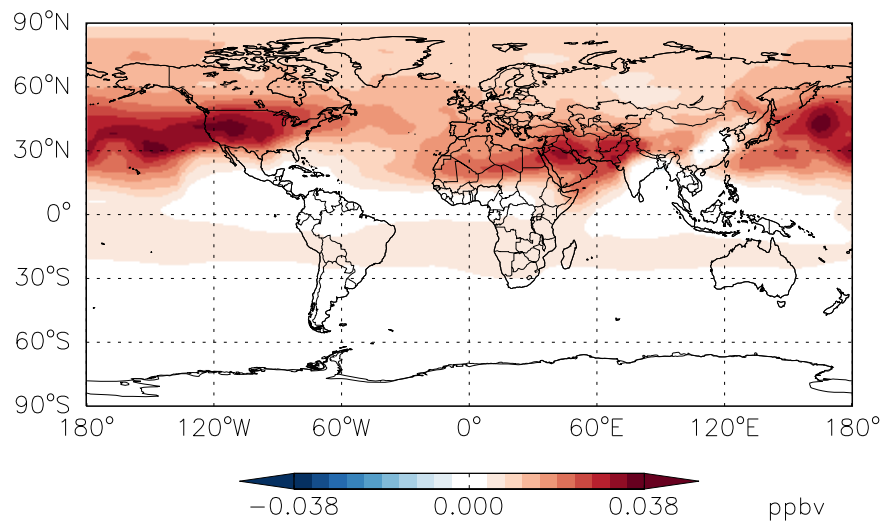
DIFF BCPI at Level 23
