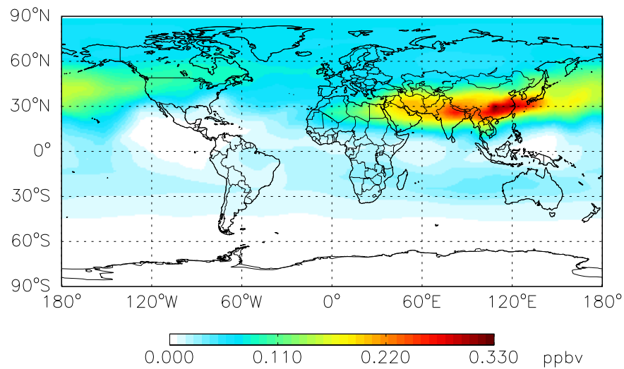
BCOC3 BCPI + BCPO at Level 30
