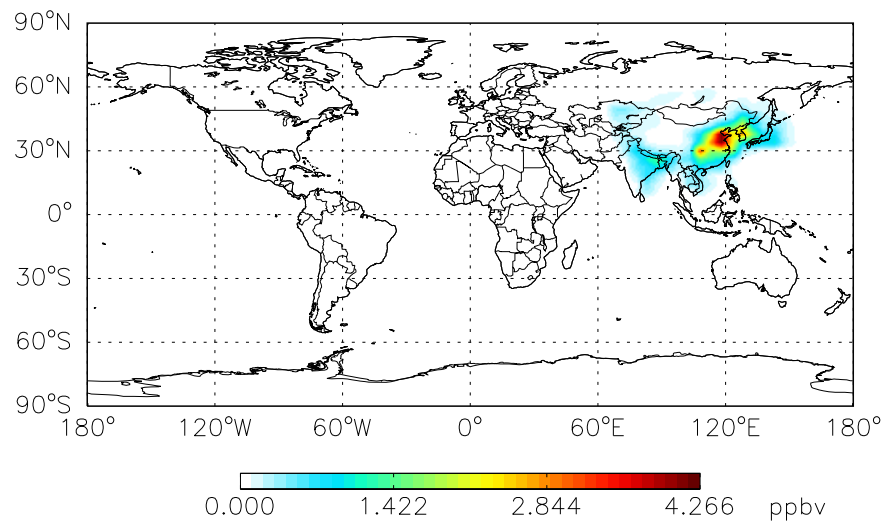
BCOC3 BCPO at Level 1
