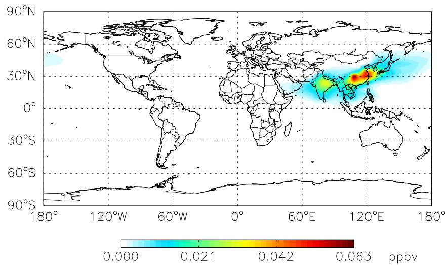
Baseline BCPO at Level 30
