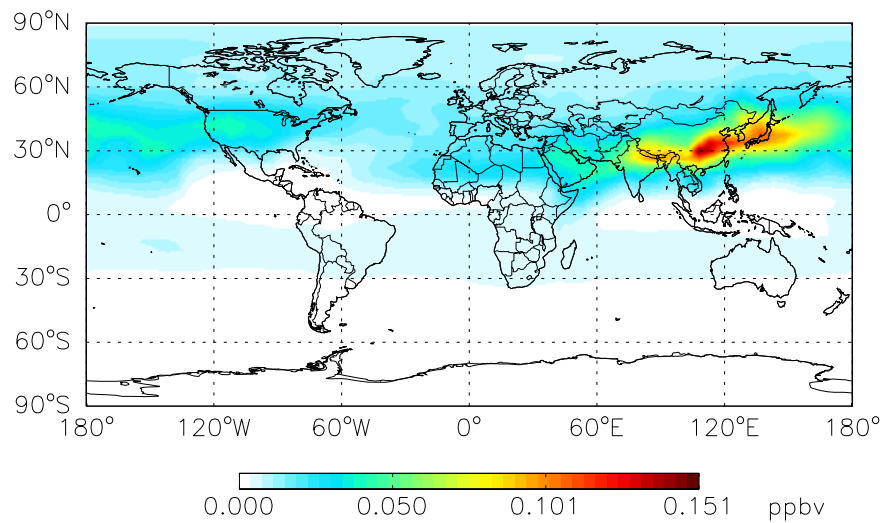
Baseline BCPI at Level 23
