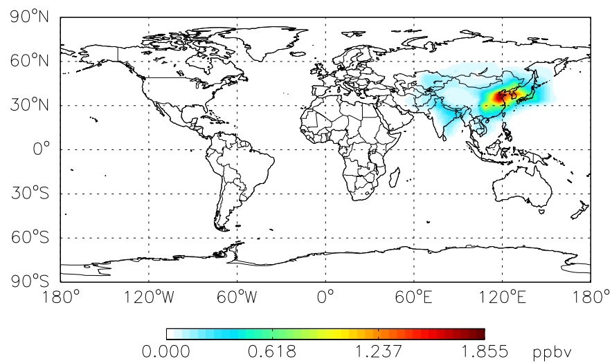
BCOC3 BCPI at Level 1
