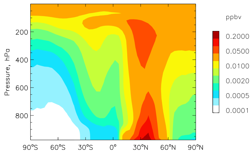
Zonal Mean – Difference BCPI + BCPO
