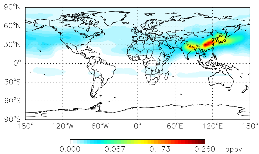
Baseline BCPI + BCPO at Level 23
