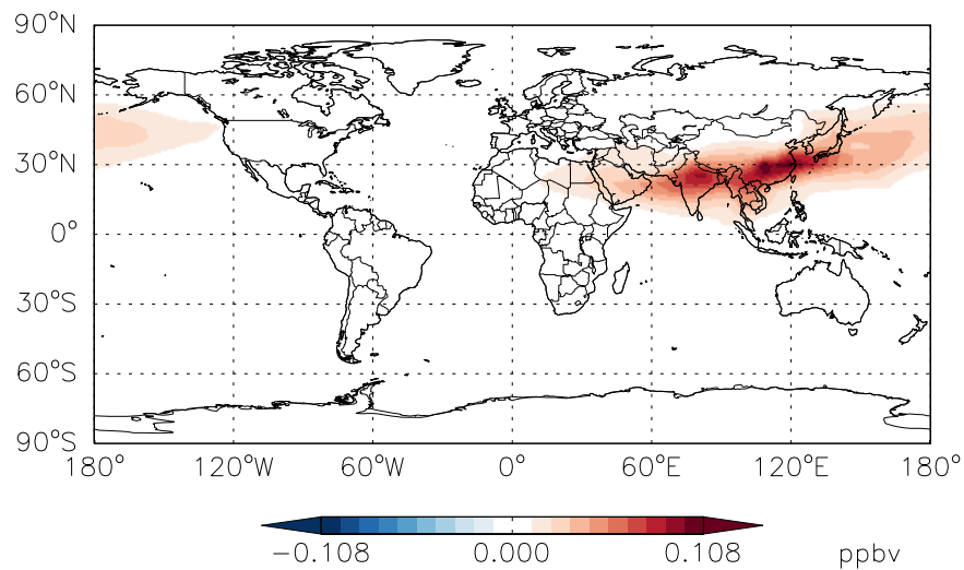
DIFF BCPO at Level 30
