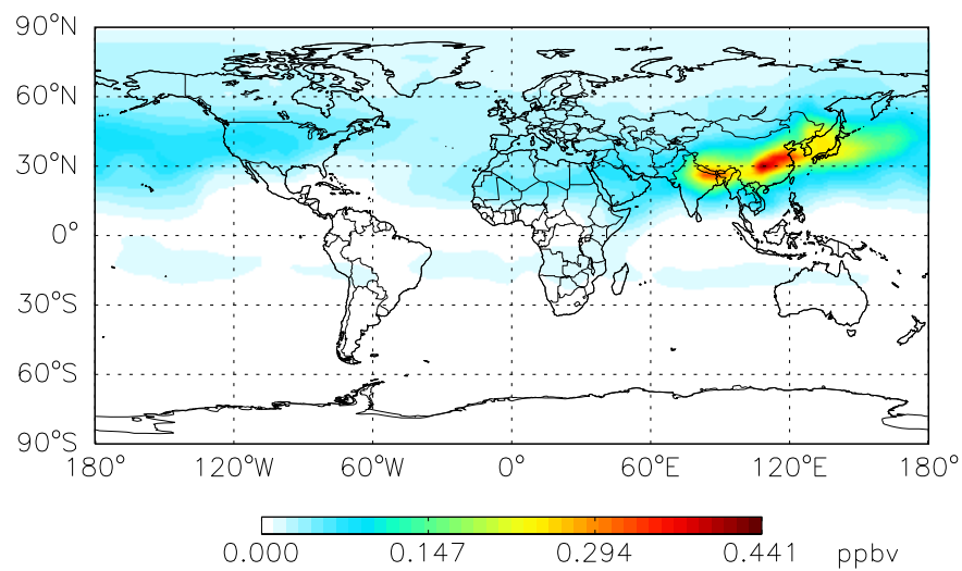
BCOC3 BCPI + BCPO at Level 23
