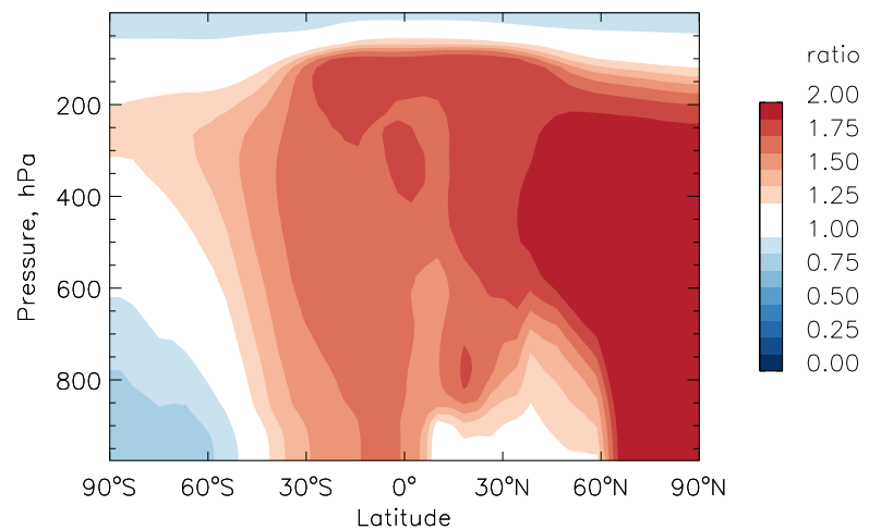
Zonal Mean – Ratio BCPI + BCPO
