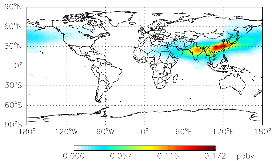
BCOC3 BCPO at Level 30
