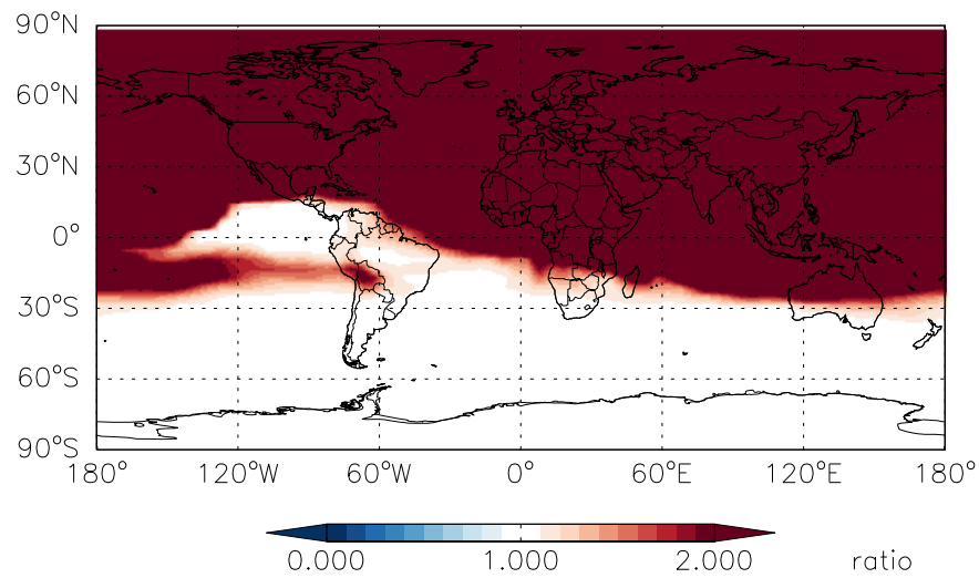
Ratio BCPO at Level 23
