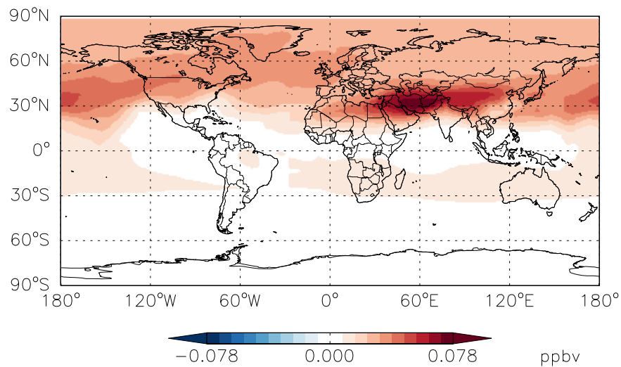
DIFF BCPI at Level 30
