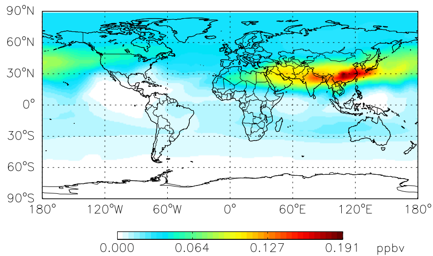
Baseline BCPI + BCPO at Level 30
