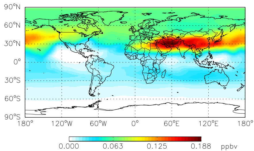
BCOC3 BCPI at Level 30
