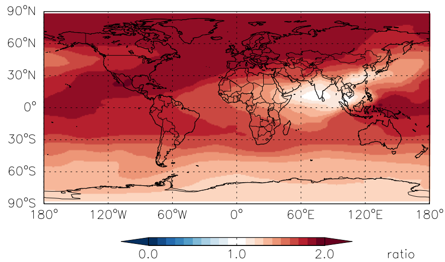
Ratio BCPI at Level 30
