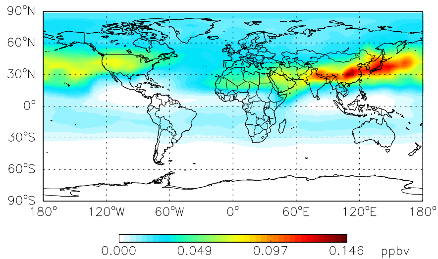
BCOC3 BCPI at Level 23
