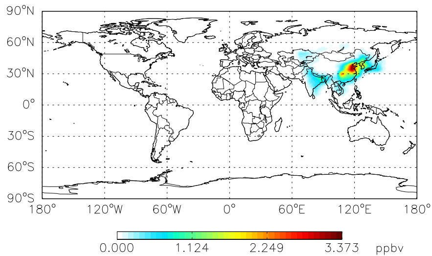
Baseline BCPO at Level 1
